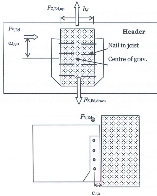
Figure B1: Definition of e_{I,90} and e_{I,0}
